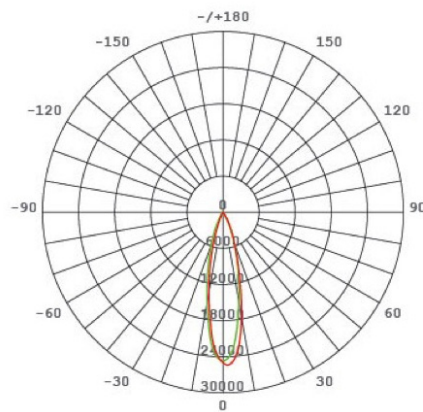
20°light distribution curve
