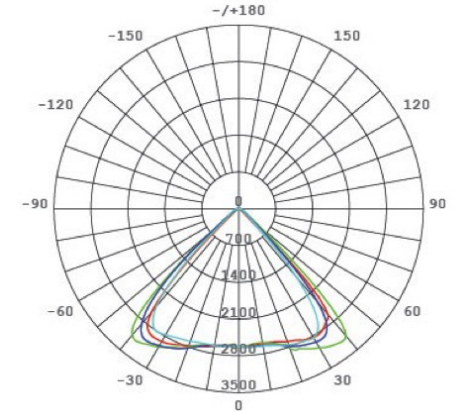
90°light distribution curve
