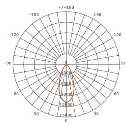
45°light distribution curve
