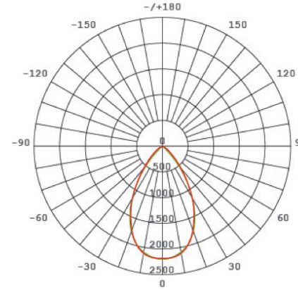
60°light distribution curve
